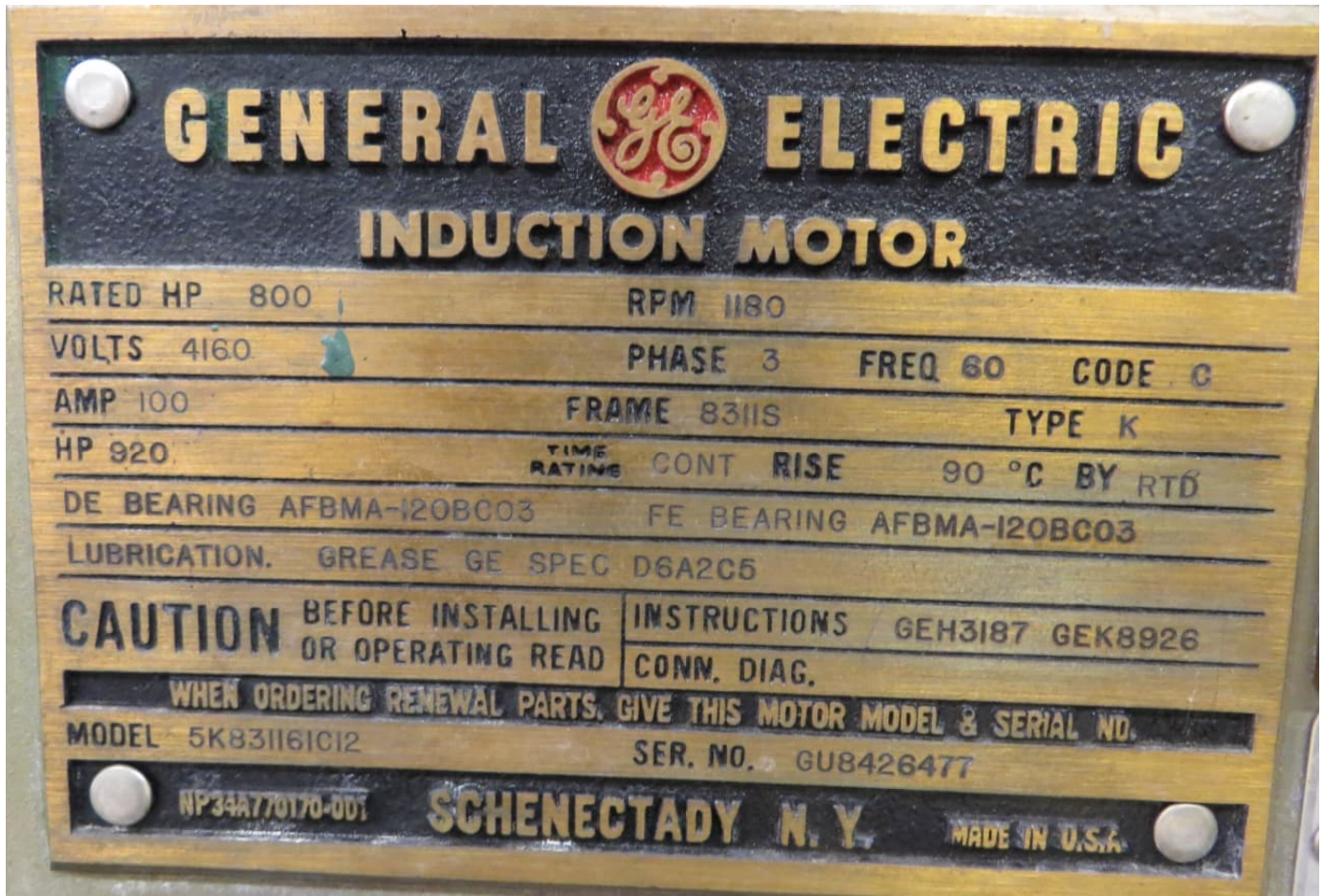
POPES HEAD PUMP STATION'S MOTOR #3 NAMEPLATE
