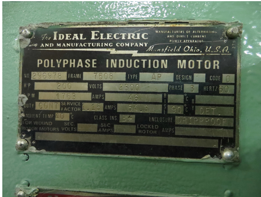
RESTON PUMP STATION'S MOTOR #2 NAMEPLATE
