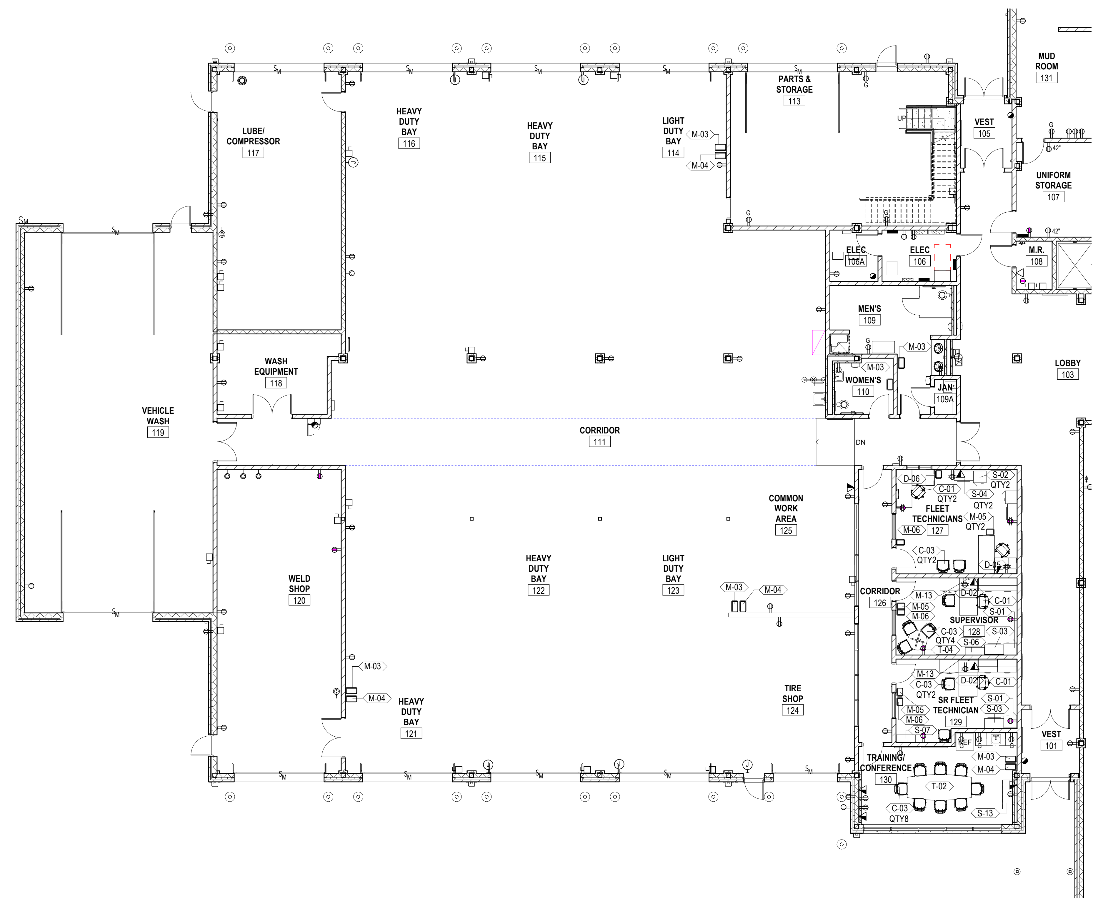
1 FIRST FLOOR FURNITURE PLAN - FLEET A-901 SCALE: 1/8" = 1'-0"
