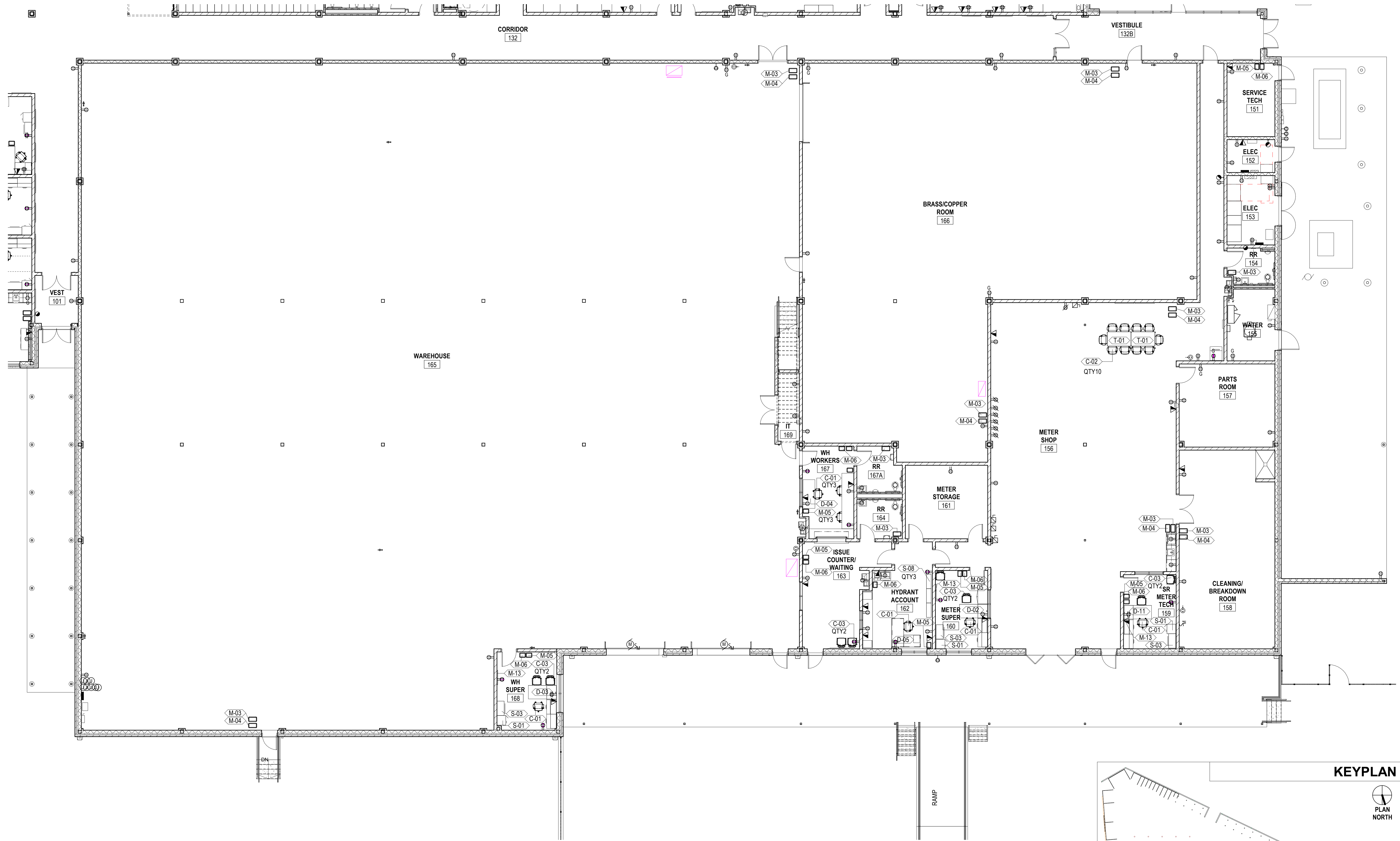
1 FIRST FLOOR FURNITURE PLAN - WAREHOUSE & METER SHOP A-900 SCALE: 1/8" = 1'-0"
